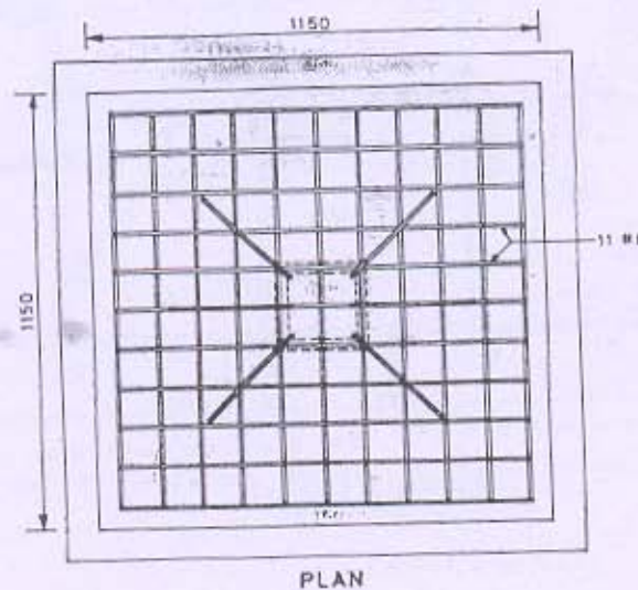
Figure 4 Q.2 (a) Column footing (column 7)
